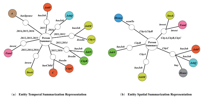
Fig. 4. The Entity Temporal Summarization and Spatial Summarization.
