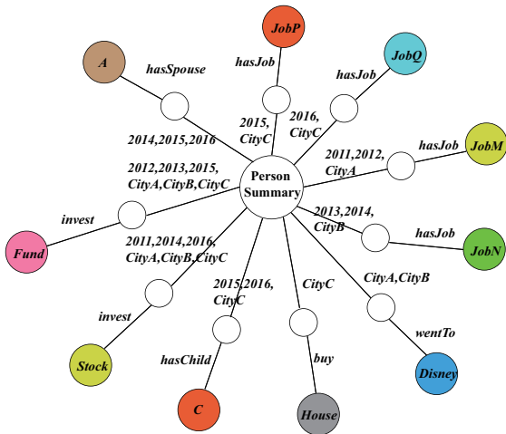
Fig. 5. The Entity Spatio-temporal Entity Summarization.
